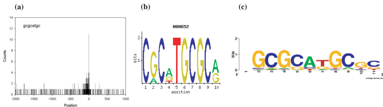
Fig. 4. Using the seed ggcgatgc , A-GLAM identified a motif in TRANSFAC corresponding to the NRF-1 factor (NF-kappaB-repressing factor). (a) Columns of the block alignments near the TSS at column 0 are shown to be enriched with occurrences of ggcgatgc . (b) Shows a sequence logo of the corresponding motif in TRANSFAC. (c) Displays the motif A-GLAM produced from the seed ggcgatgc .
