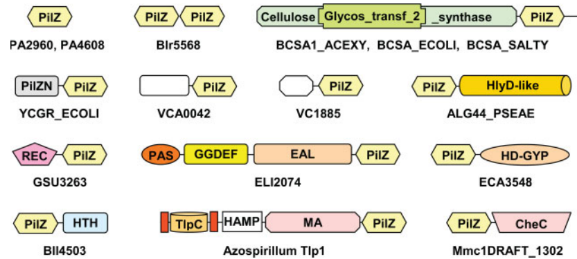
Fig. 2. Domain architectures of selected PilZ-containing proteins. The first two rows show the most common domain structures, the last two rows show rare domain combinations that indicate involvement of PilZ in signaling. Proteins are listed by UniProt entry names or their gene names. Source organisms and GenBank/EMBL protein accession numbers are as follows: PA2960 and PA4608, Pseudomonas aeruginosa AAG06348 and AAG07996, respectively; Blr5568 and Bll4503, Bradyrhizobium japonicum BAC50833 and BAC49768; VCA0042 and VC1885, Vibrio cholerae AAF95956 and AAF95033; GSU3263, Geobacter sulfurreducens AAR36654; ELI2074, Erythrobacter litoralis EAL74814; ECA3548, Erwinia carotovora CAG76446; Mmc1draft_1302, Magnetococcus sp. MC-1 EAN28119. Domain designations are as follows: Cellulose synthase, Pfam domain PF03552; Glycos_transf_2, PF00535; PilZN and PilZNR, new domains that will be described elsewhere; HlyD-like, a divergent variant of the PF00529 domain; REC, PF00072; PAS, PF0989; GGDEF, PF00990; EAL, PF00563; HD-GYP, COG2206, a variant of PF01966 (Galperin et al. , 1999); HTH_3, PF01381; TlpC, a periplasmic signaling domain (Greer-Phillips et al. , 2004); HAMP, PF00672; MCPsignal, PF00015; CheC, COG1776, a protein phosphatase domain (Park et al. , 2004).
