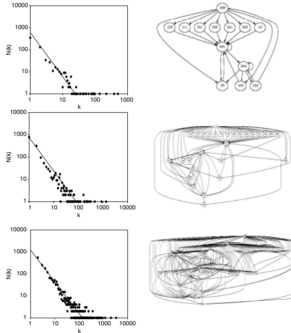
Fig. 2. Plots showing the effect of the threshold parameter on the size of a network and on the scaling of node degrees. Strongly coupled components of networks at various thresholds \epsilon (right-hand side). Plot of degree distribution, N(k) versus k for diauxic shift data at different thresholds (left-hand side). Plots show that scaling is independent of threshold value. Actual thresholds differ somewhat between left- and right-hand examples. Threshold was varied by a factor of 2 to generate scaling plots. The lines in right-hand plots represent functions with a slope of -3/2 . Note that they intersect the axes at different points, however, reflecting the different numbers of nodes in the graphs. Graphs derived from the cdc data of Spellman et al. (1998) .
