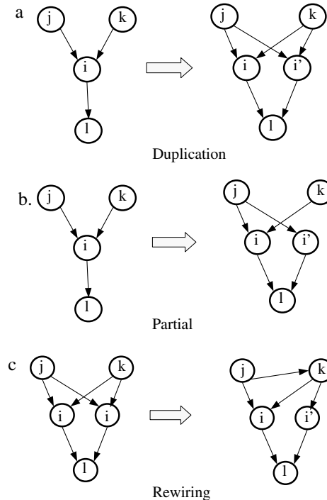
Fig. 1. Schematic representation of network growth through gene duplication. (a) Shows pure gene duplication where a new node is created by duplicating the connectivity of the parent. This results in an increase in degree of the neighboring nodes. Node i is duplicated to give i' . Nodes j, k, l are neighbors. (b) The partial duplication model where node i is duplicated to i' but not all the original connections are retained. (c) Shows a rewiring process where edge i-j is rewired to become i-k .
