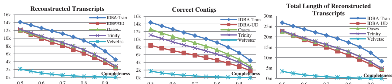
Fig. 5. Experiment result of each assembler on different completeness level for real data
